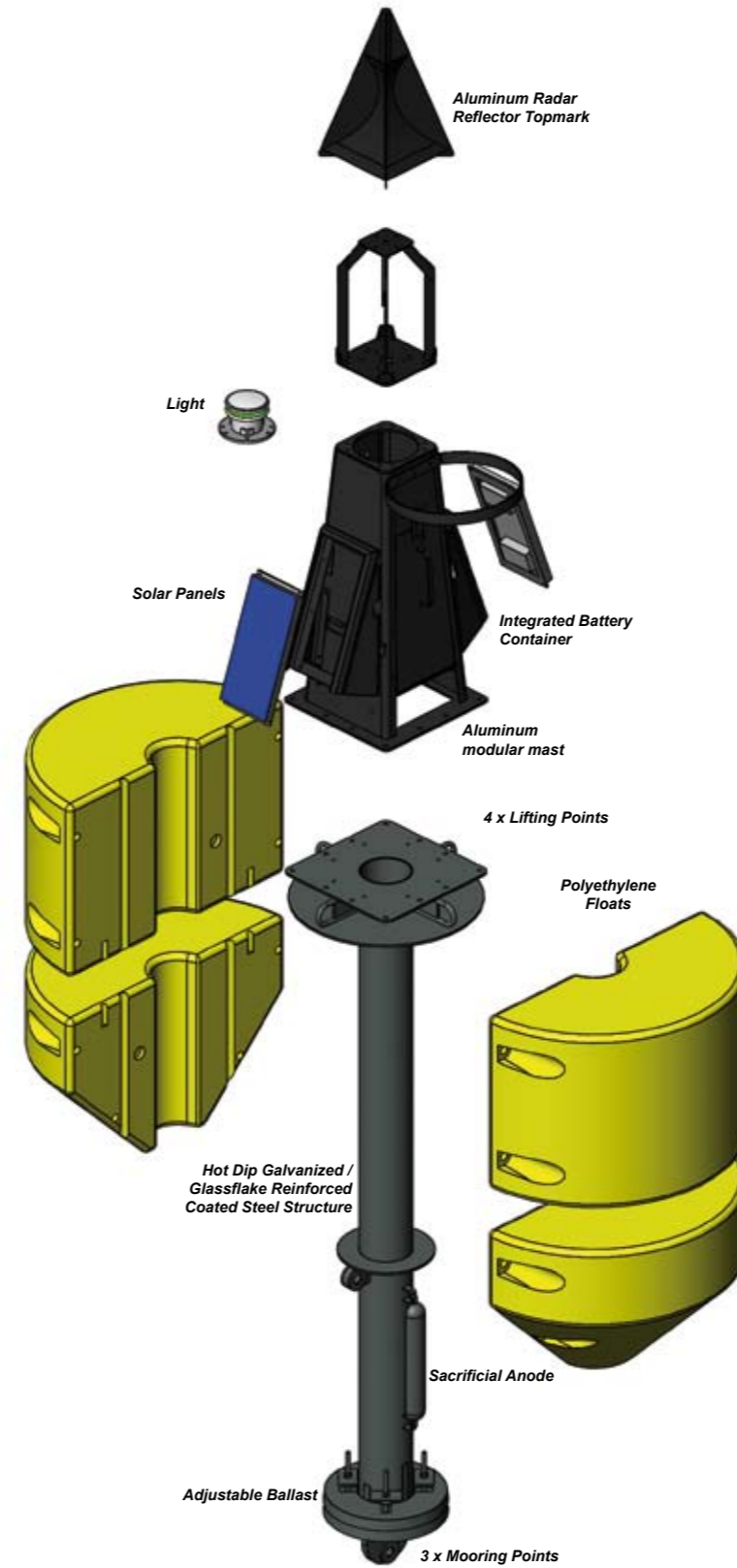
Exploded view of a AQ 1500 Anchoring elements (shackles, chains, swivels, sinkers) are available in mooring device section in catalogue
